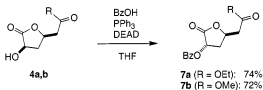
Scheme 3. Mitsunobu reactions of 4a and 4b
