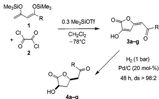
Scheme 1. Synthesis of \gamma -butyrolactones 4a–g
