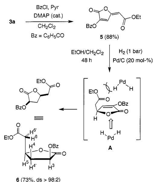
Scheme 2. Synthesis and structure elucidation of lactone 6
