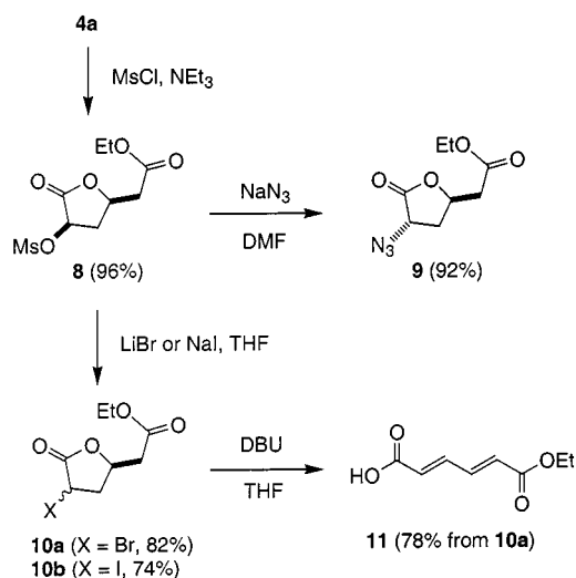
Scheme 4. Functionalization reactions of lactone 4a
