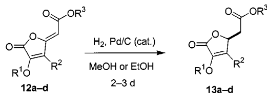
Scheme 5. Hydrogenation of butenolides 12a–d
